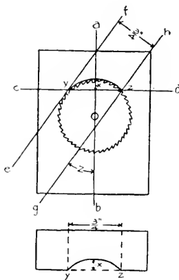
FIG. 171. CUTTING CORE BOX ON UNIVERSAL SAW TABLE.
